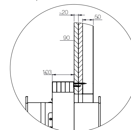
FD25, FD40 - side cross section
