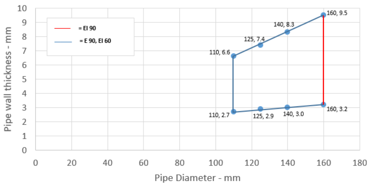
PVC Pipes 110-160 / 50 mm Collar - U/C
