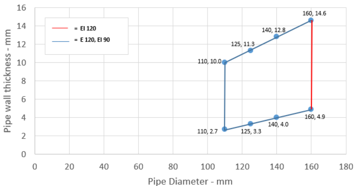
PP Pipes 125-160 / 60 mm collar - C/C
